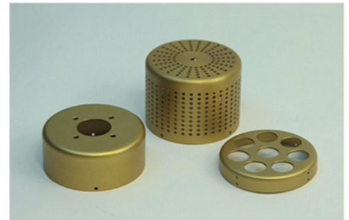
Gold Anodized 0.040" Aluminum, electrical housing, three piece assembly. 3.00" diameter X 4.00" height.
